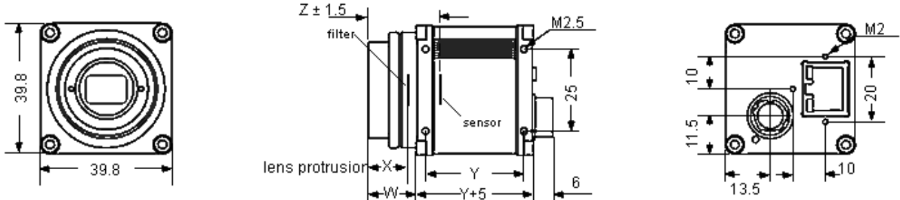
Dimensions in mm W = approx. 10 (CS mount) | 15 (C mount), Y = 30 (remaining sensors) X = 6 (CS mount) | 8 (C mount), Z = 12.5 (CS mount) | 17.526 (C mount)
