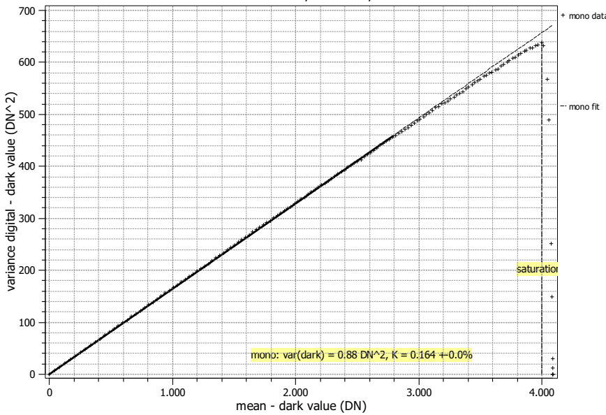
Photon transfer m0749, 536 nm, 07.12.2018
