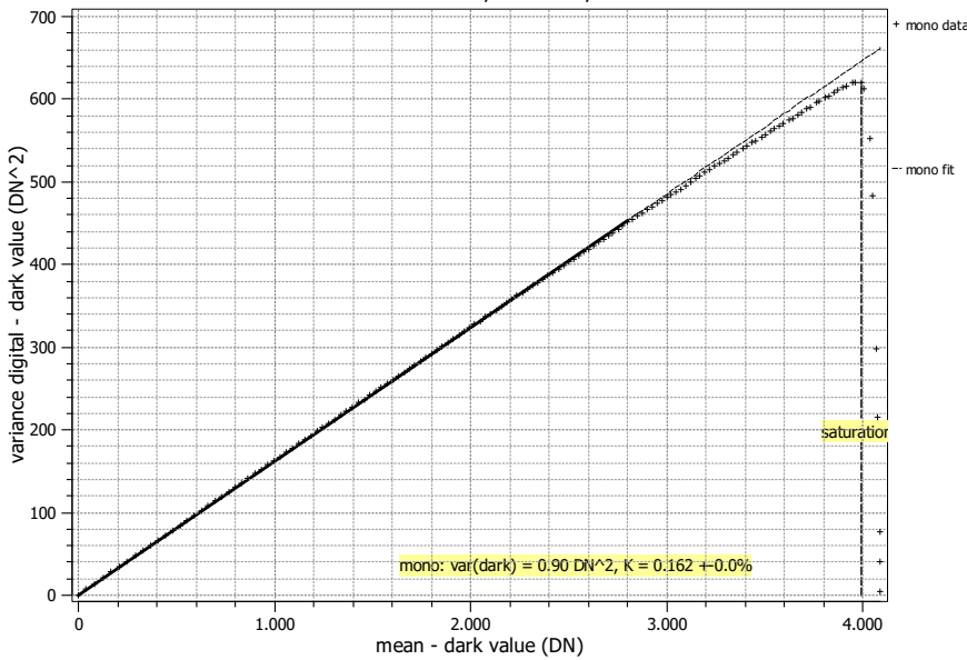
Photon transfer m0801, 535 nm, 02.05.2019
